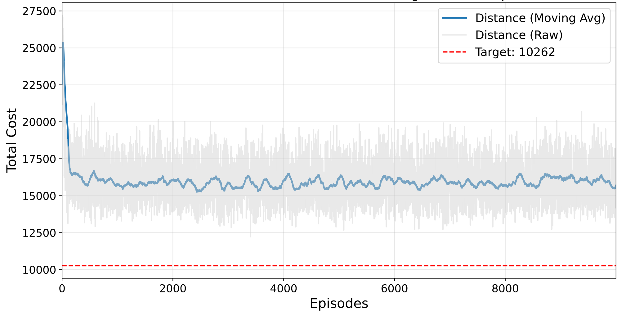
Final Masked AutoRL-SOP Training - ft53.3.sop
